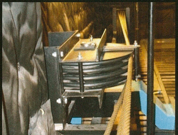
Heavy Duty Divert Pulley
