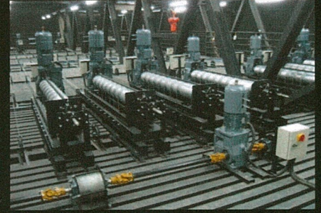
Fly-bar Machinery & Bar Hoist
